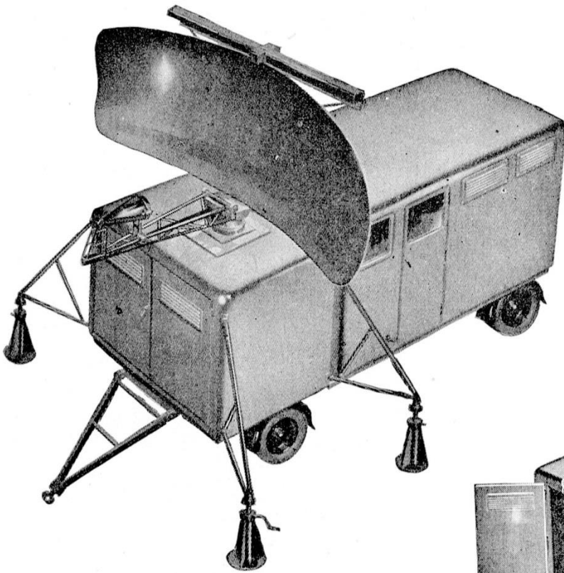
The Aerial Head, jack-supported, is suitable for mobile, tower or roof mounting. A Secondary Radar aerial can be mounted on top of the scanner, as shown here.
